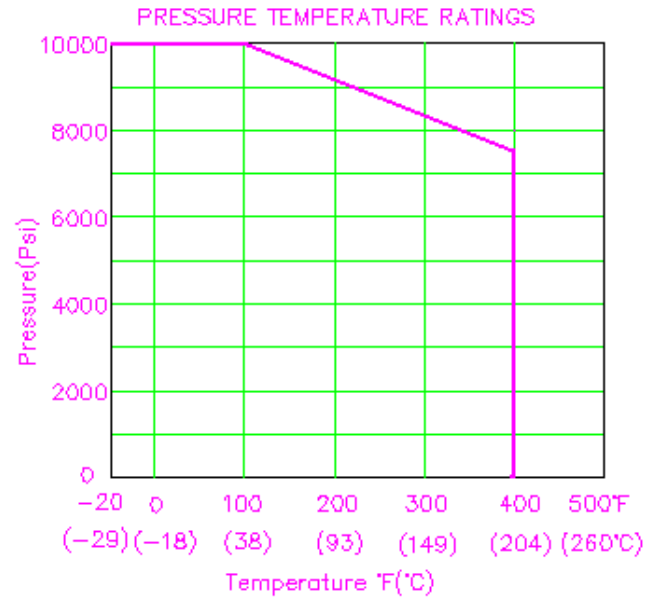
Needle Valves
